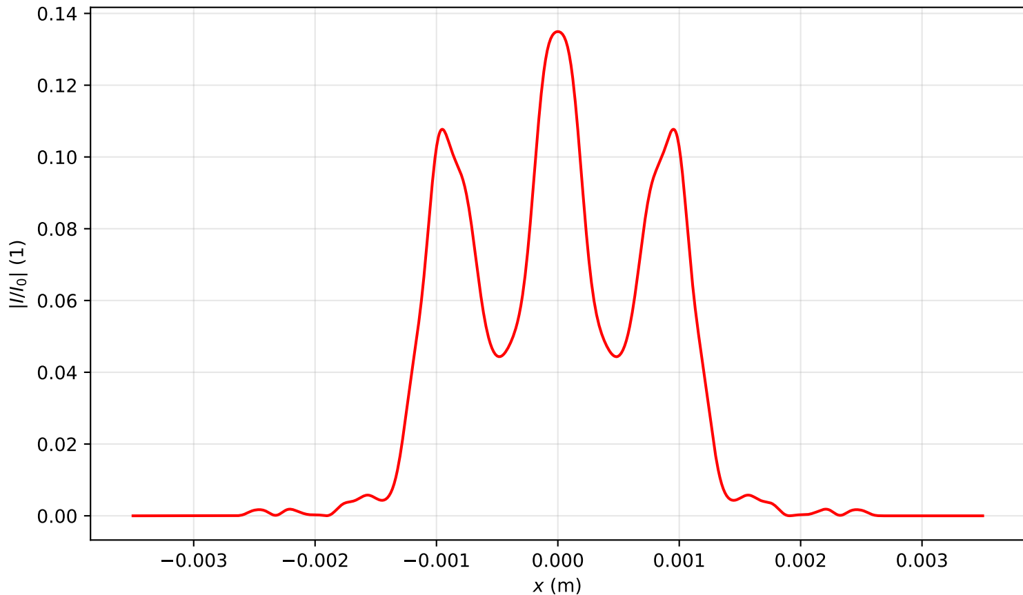
Intensity profile I(x, y = 0, z = 2.388)/I_0 , P_{in}=6.5P_{cr} , artificial time
